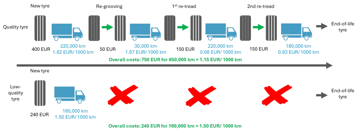
Figure 22. Tyre as a service business model that utilises tyre re-grooving and retreading (Marangoni, 2024).
