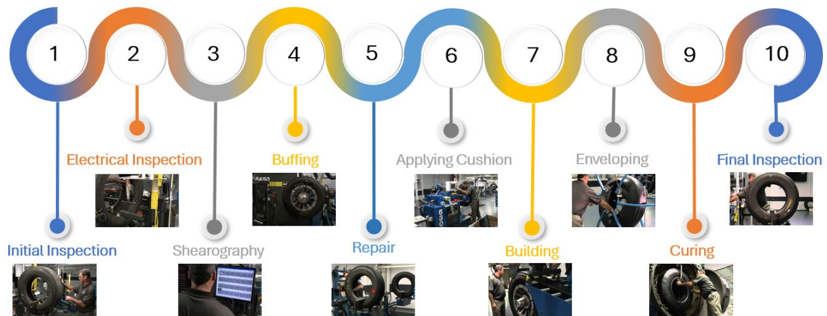
Figure 21. Retreading process used by Bandag (Adapted from Bridgestone, 2024).
