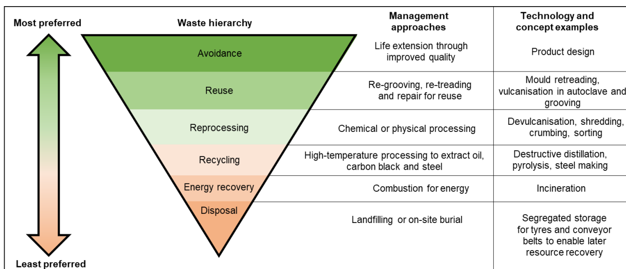
Figure 27. Tyre management approaches and technologies mapped against the waste hierarchy.
