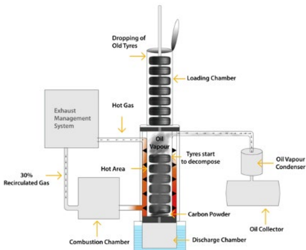
Figure 26. Green Distillation Technology (Destructive distillation) process overview, based on (Green Distillation Technologies Corporation LTD, 2024; Hossain et al., 2020).
