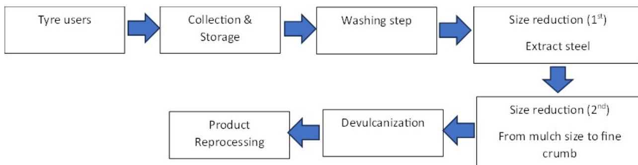
Figure 23. Process flow for devulcanisation technology (Drawn based on personal communication, 2023).
