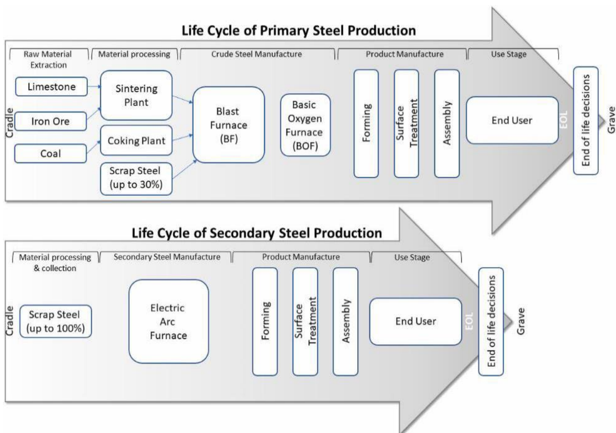
Figure 24. Typical steel making processes (Davies and Hastings, 2022)
